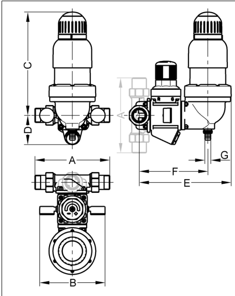
Fig. 8: Installing dimensions JPM 1½" - 2"
