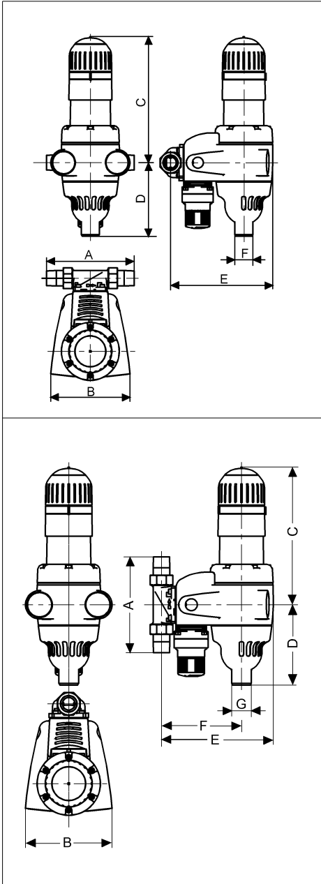
Fig. 7: Installing dimensions JPM 3/4" - 1 1/4"
