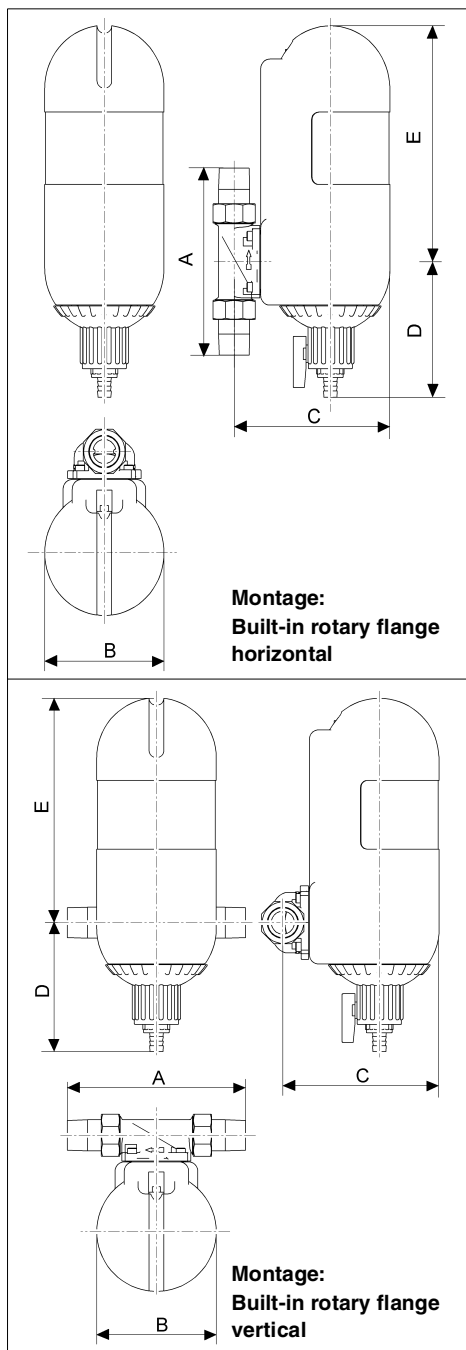
Fig. 6: Installed dimensions \frac{3}{4} " - 1\frac{1}{4} "
