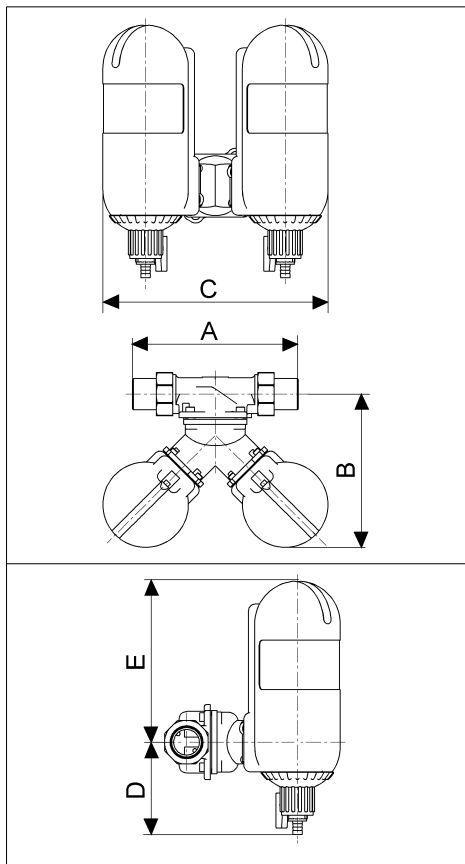
Fig. 7: Installed dimensions 1½" - 2"
