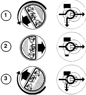
Fig. 5: Backwashing
