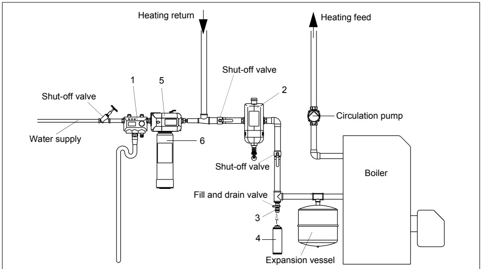
Fig. 2: Schematic JUDO MAFI with fixed heating water conditioning according to VDI 2035
