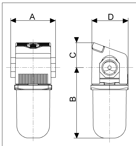
Illustration 1: Cotes de montage MHF
